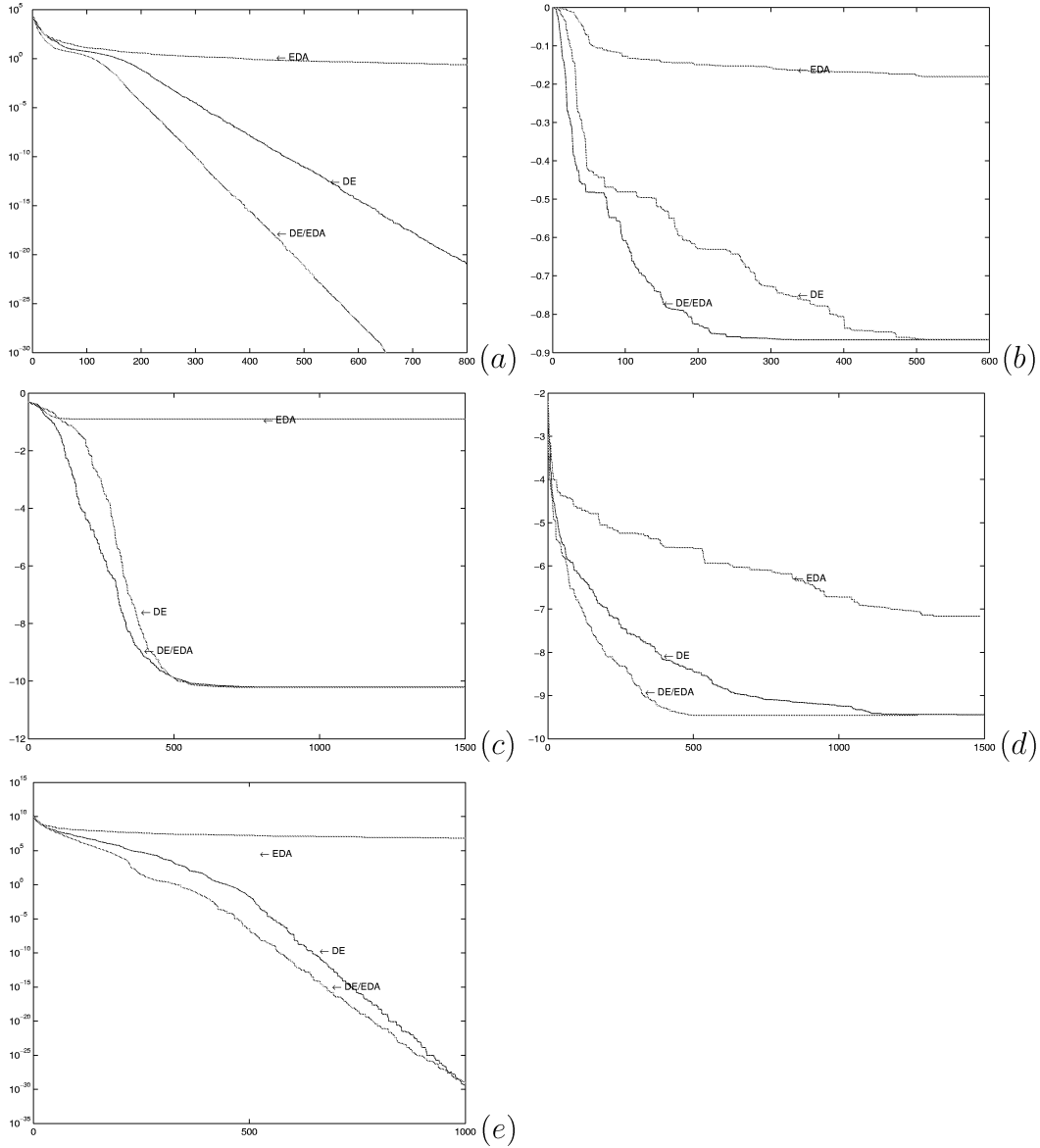
Fig. 2. The evolution procedure for solving problems with dimension 10.
