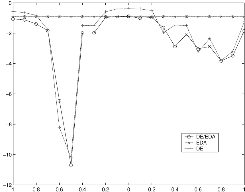
Fig. 3. The effect of F to the performance of DE/EDA taking the Shekel's Foxholes as an example.
