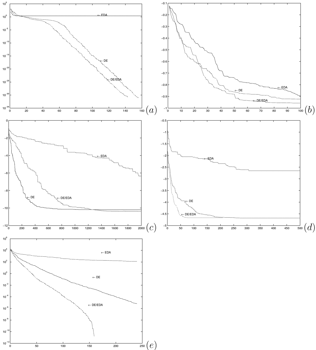
Fig. 1. The evolution procedure for solving problems with dimension 5.
