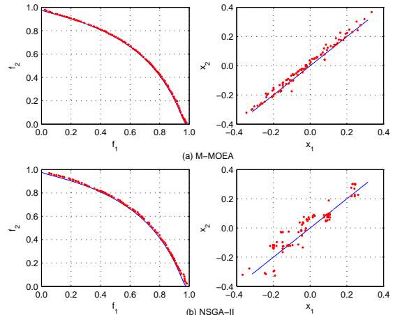
Figure 7: The results on FON
