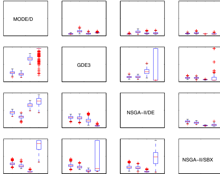
Fig. 2. The box plots of \mathcal{C} -metric of MODE/D, GDE3, NSGA-II/DE, and NSGA-II/SBX. Four box plots from left to right in each chart relate to OKA-1, OKA-2, ZDT1-L, and ZDT-L, respectively.
