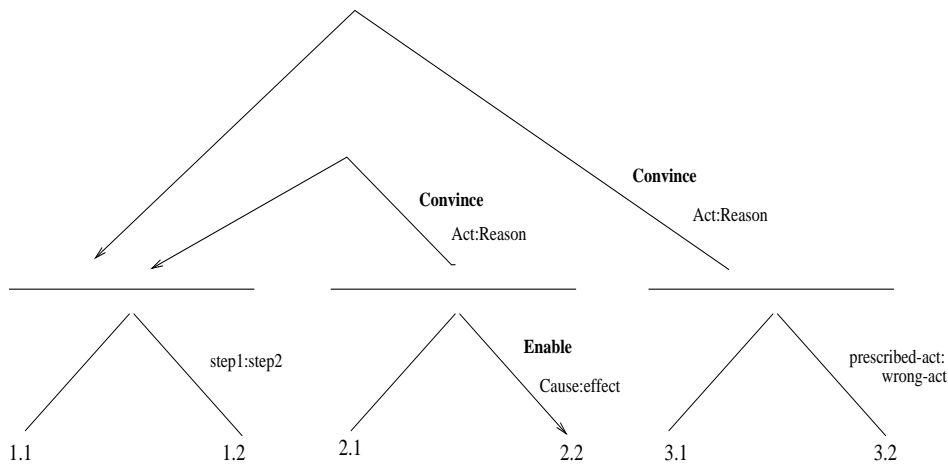
Figure 1.1: A tutorial excerpt and its RDA analysis
