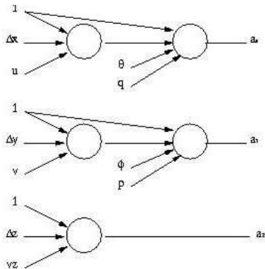
Figure 3: Neural controller. Arrows indicate variable weight synaptic connections, and nodes compute the tanh of the sum of their inputs.
