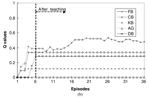
Fig. 13. The Q value changes in two feature states during the Q-learning.
